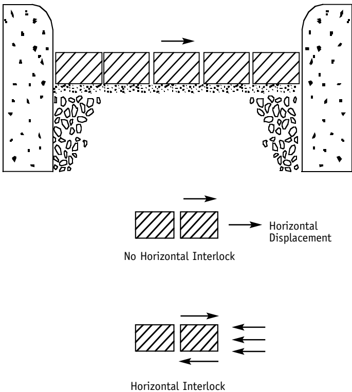
Figure 4: Horizontal Interlock
