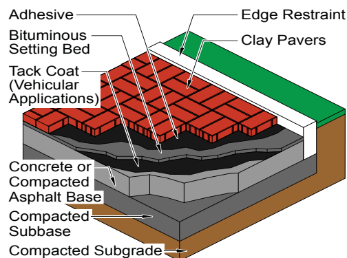
Figure 1 Typical Brick Pavement on Bituminous Setting Bed
